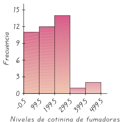
FIGURA 2-1 Histograma
