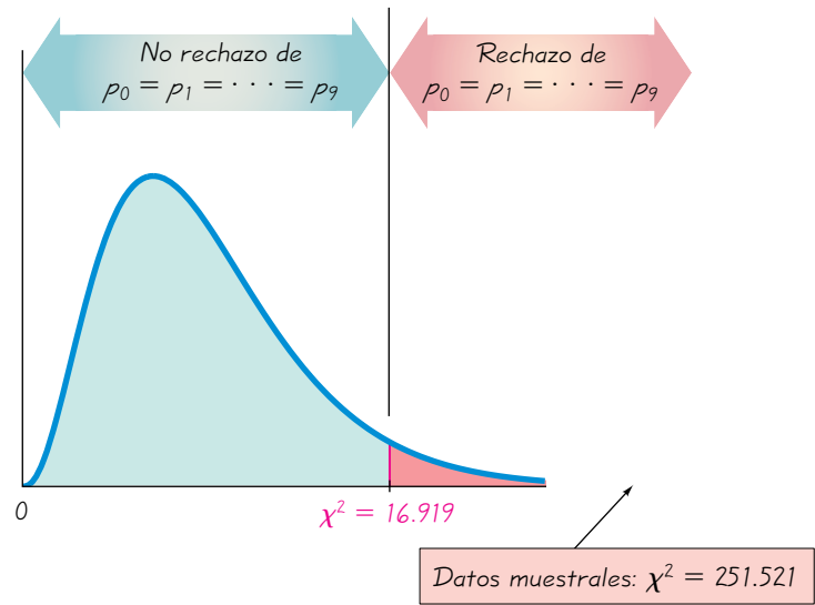
FIGURA 10-4 Prueba de p_0 = p_1 = p_2 = p_3 = p_4 = p_5 = p_6 = p_7 = p_8 = p_9
