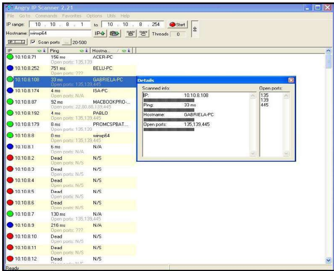
Figura 4.24 Angry IP Scanner - Escaneo de Host Vivos - Windows.
